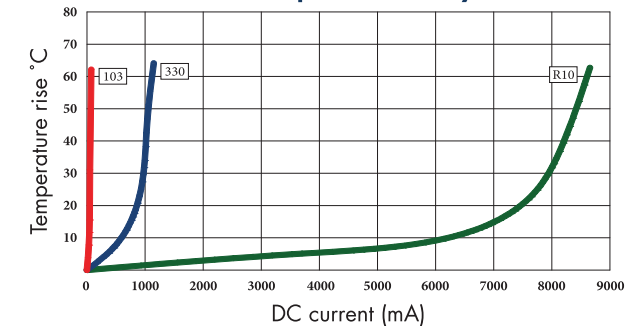
OWI2220 Temperature rise by current
