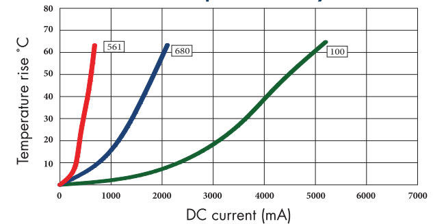
OWI104 Temperature rise by current
