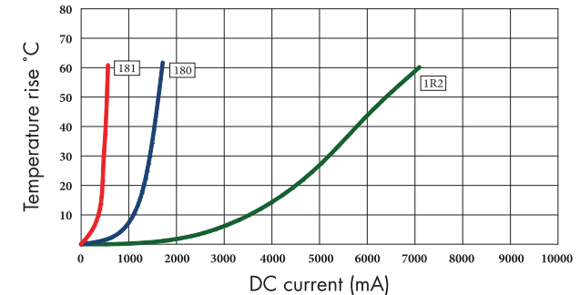
OWIRH4D28 Temperature rise by current
