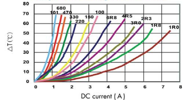
Temperature Change vs. DC Current
