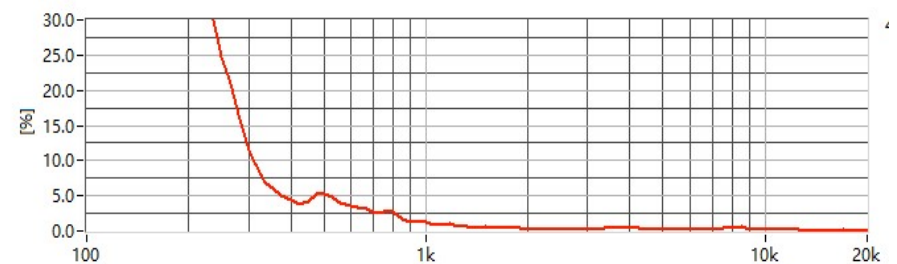
Total Harmonic Distortion
