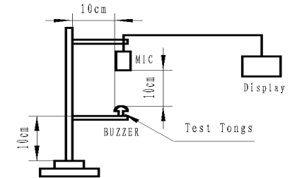
Test Equipments
